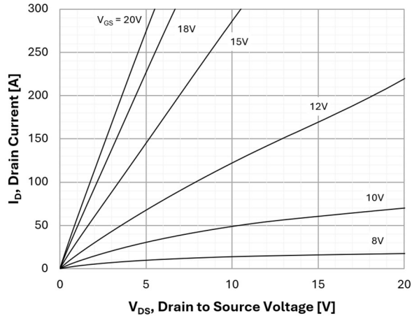
Figure 3. On-Region Characteristics
