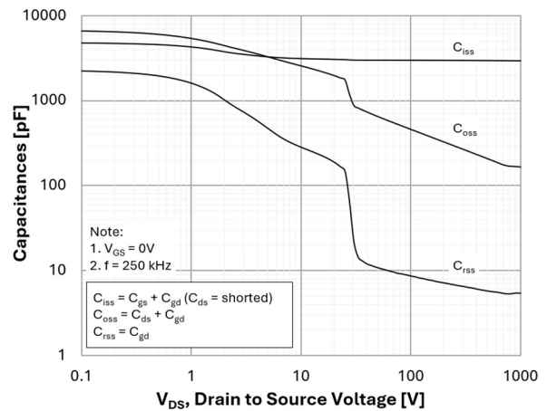
Figure 12. Capacitance Characteristics
