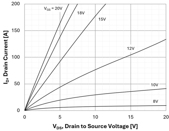
Figure 3. On-Region Characteristics
