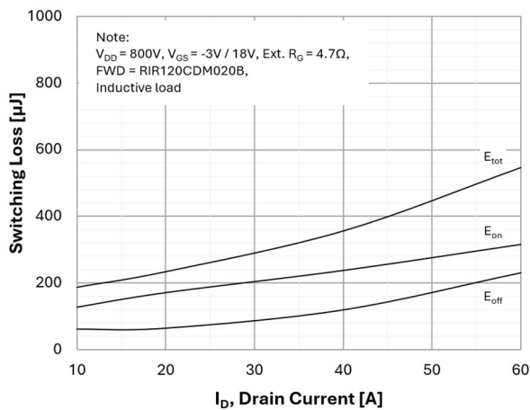
Figure 15. Typical Switching Losses vs. Drain Current
