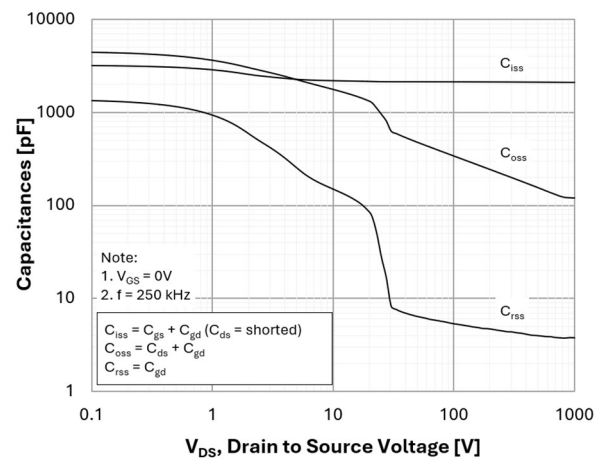
Figure 12. Capacitance Characteristics
