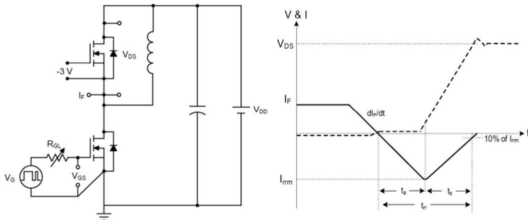
Figure 22. Peak Diode Recovery dI_F/dt Test Circuit and Waveforms
