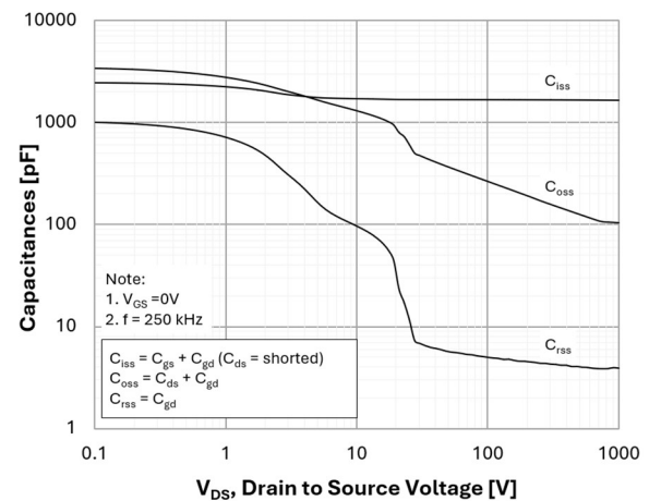
Figure 12. Capacitance Characteristics
