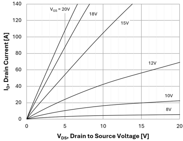
Figure 3. On-Region Characteristics
