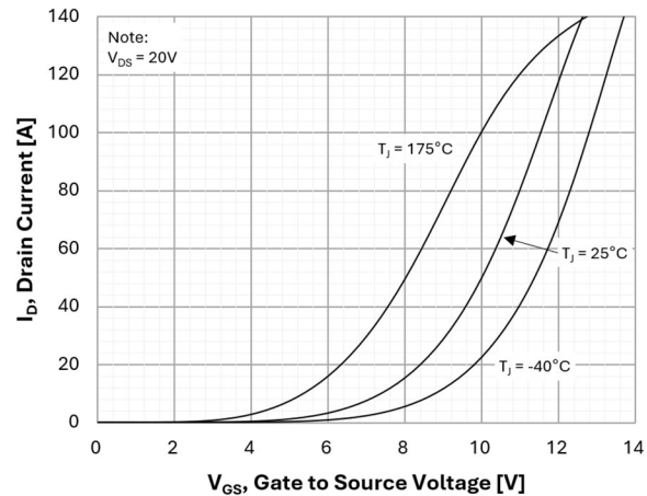
Figure 5. Transfer Characteristic
