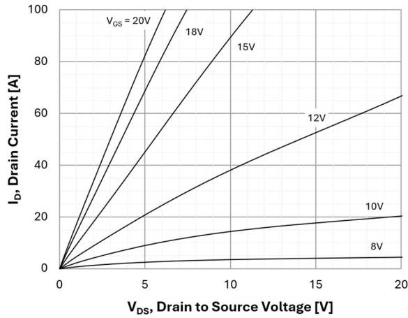
Figure 3. On-Region Characteristics
