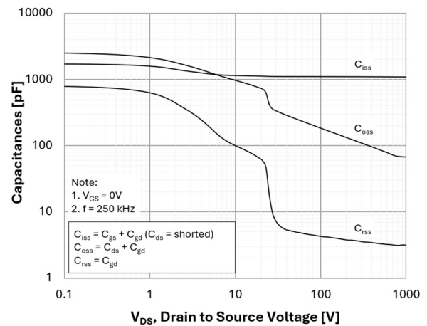
Figure 12. Capacitance Characteristics
