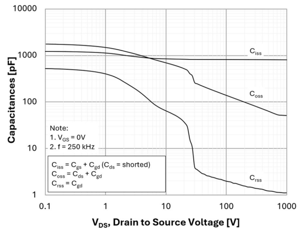
Figure 12. 2 Capacitance Characteristics
