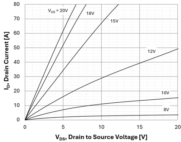
Figure 3. On-Region Characteristics
